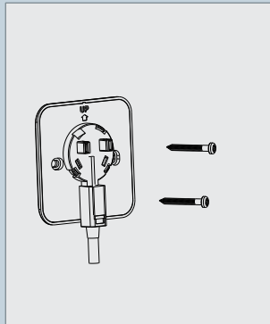
2 Install the backplate onto the wall.
