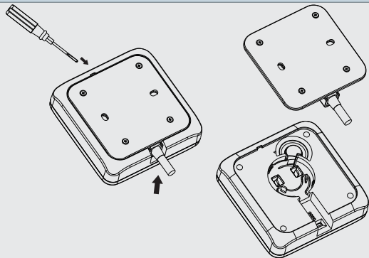
1 Open backplate from the top
